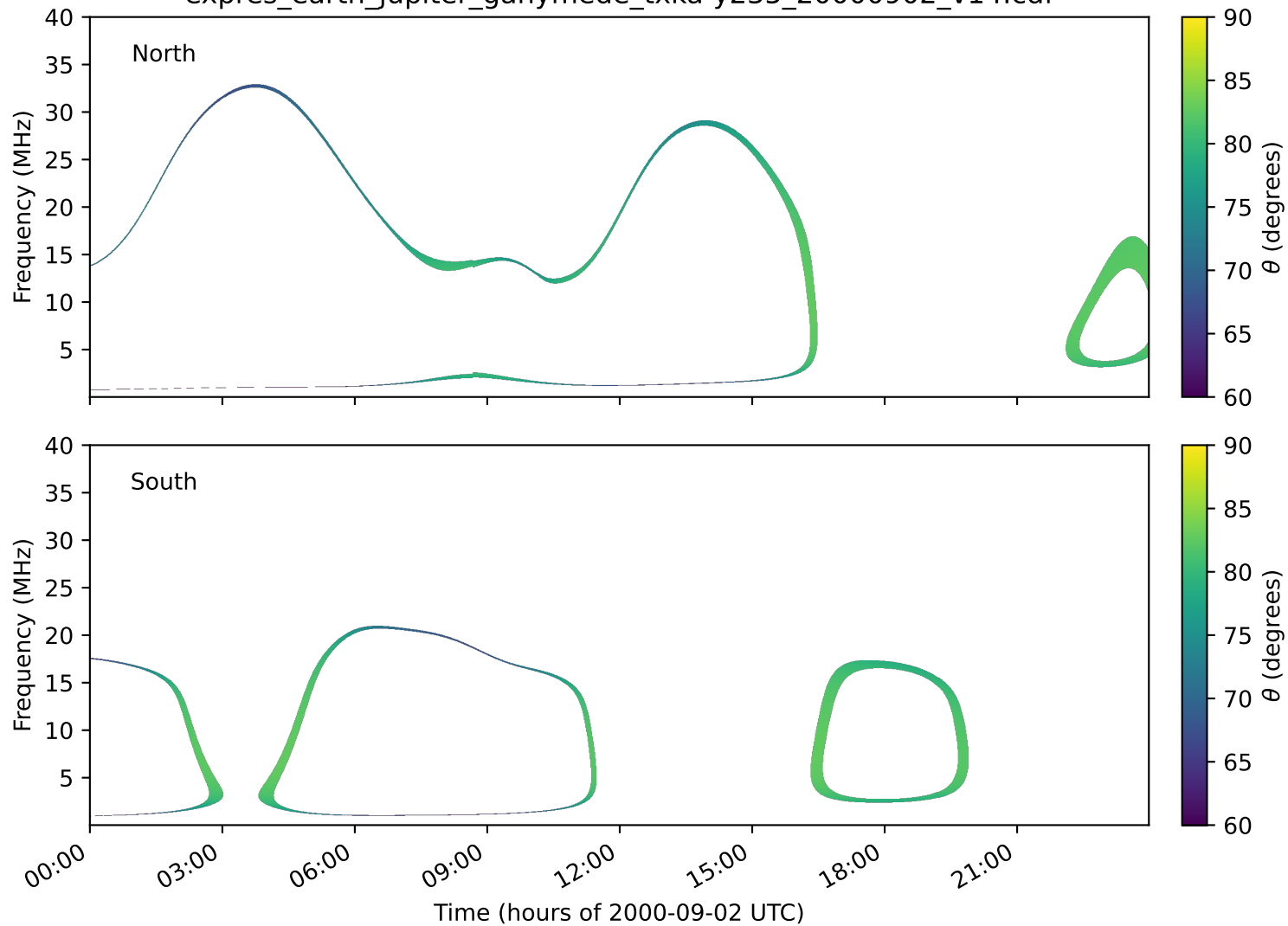
expres_earth_jupiter_ganymede_txka-y235_20000902_v14.cdf
