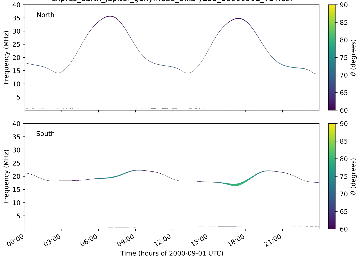
expres_earth_jupiter_ganymede_txka-y235_20000901_v14.cdf
