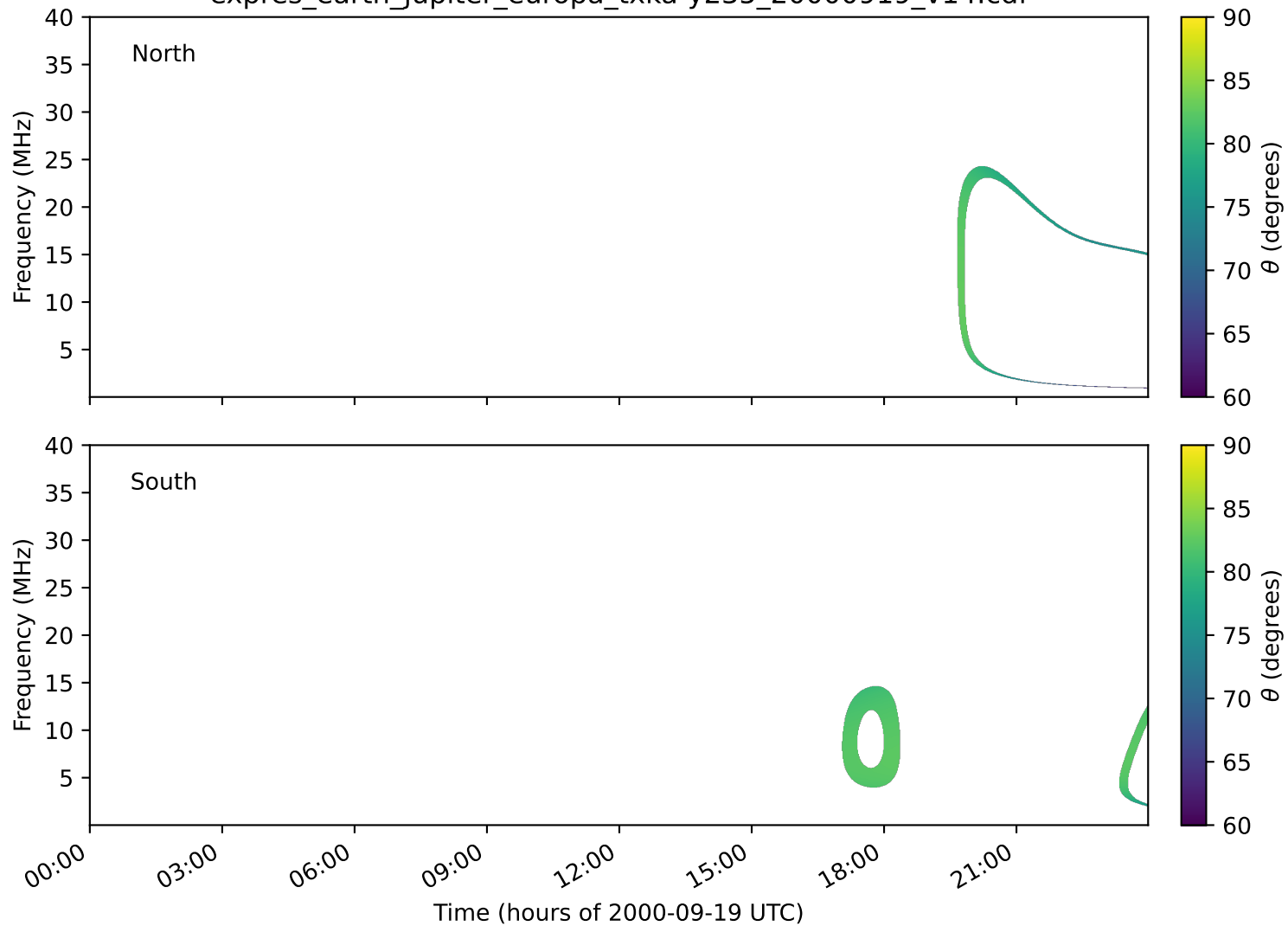
expres_earth_jupiter_europa_txka-y235_20000919_v14.cdf
