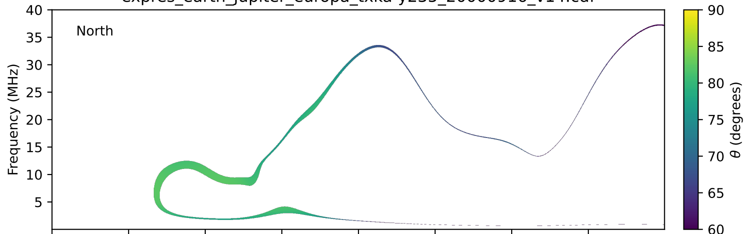
expres_earth_jupiter_europa_txka-y235_20000916_v14.cdf
