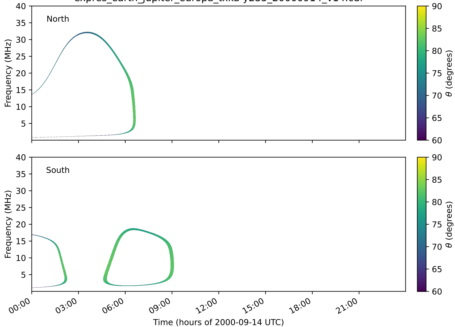
expres_earth_jupiter_europa_txka-y235_20000914_v14.cdf
