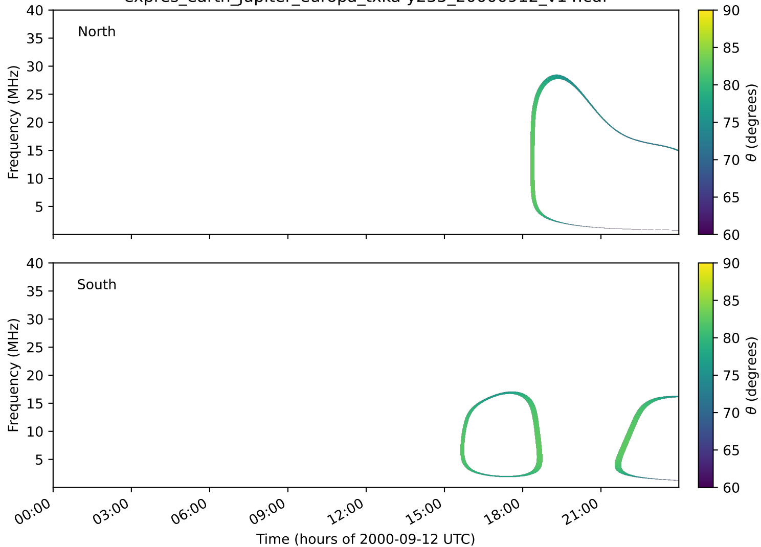
expres_earth_jupiter_europa_txka-y235_20000912_v14.cdf
