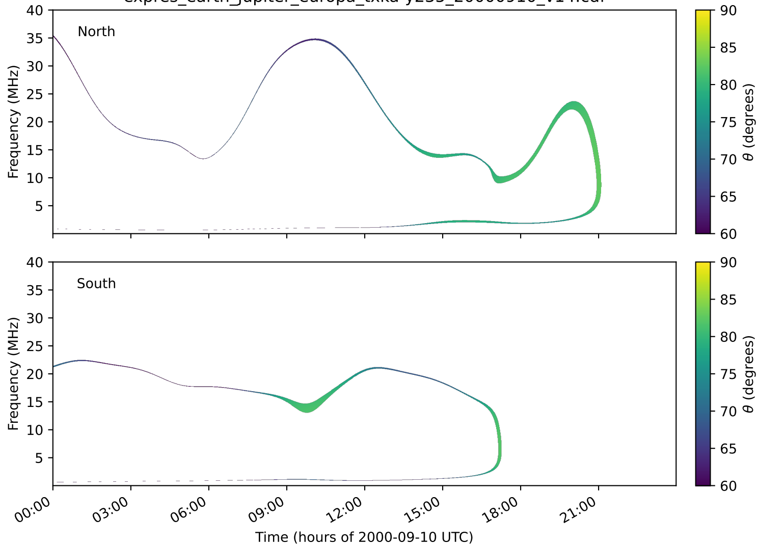
expres_earth_jupiter_europa_txka-y235_20000910_v14.cdf
