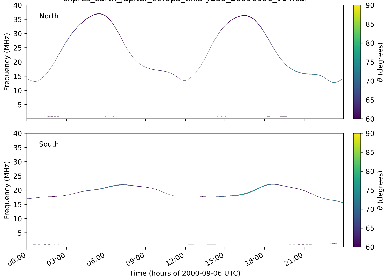
expres_earth_jupiter_europa_txka-y235_20000906_v14.cdf
