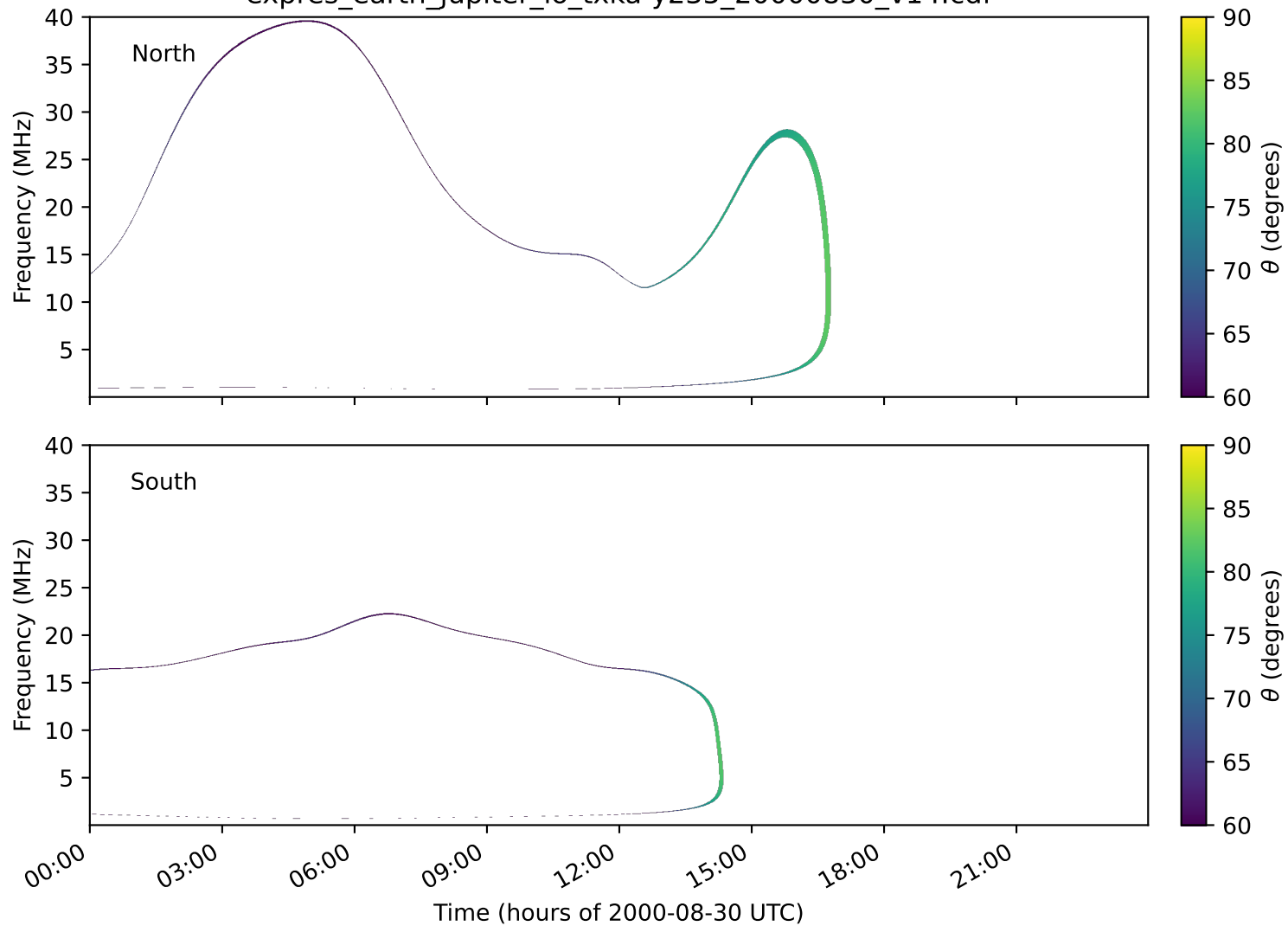
expres_earth_jupiter_io_txka-y235_20000830_v14.cdf
