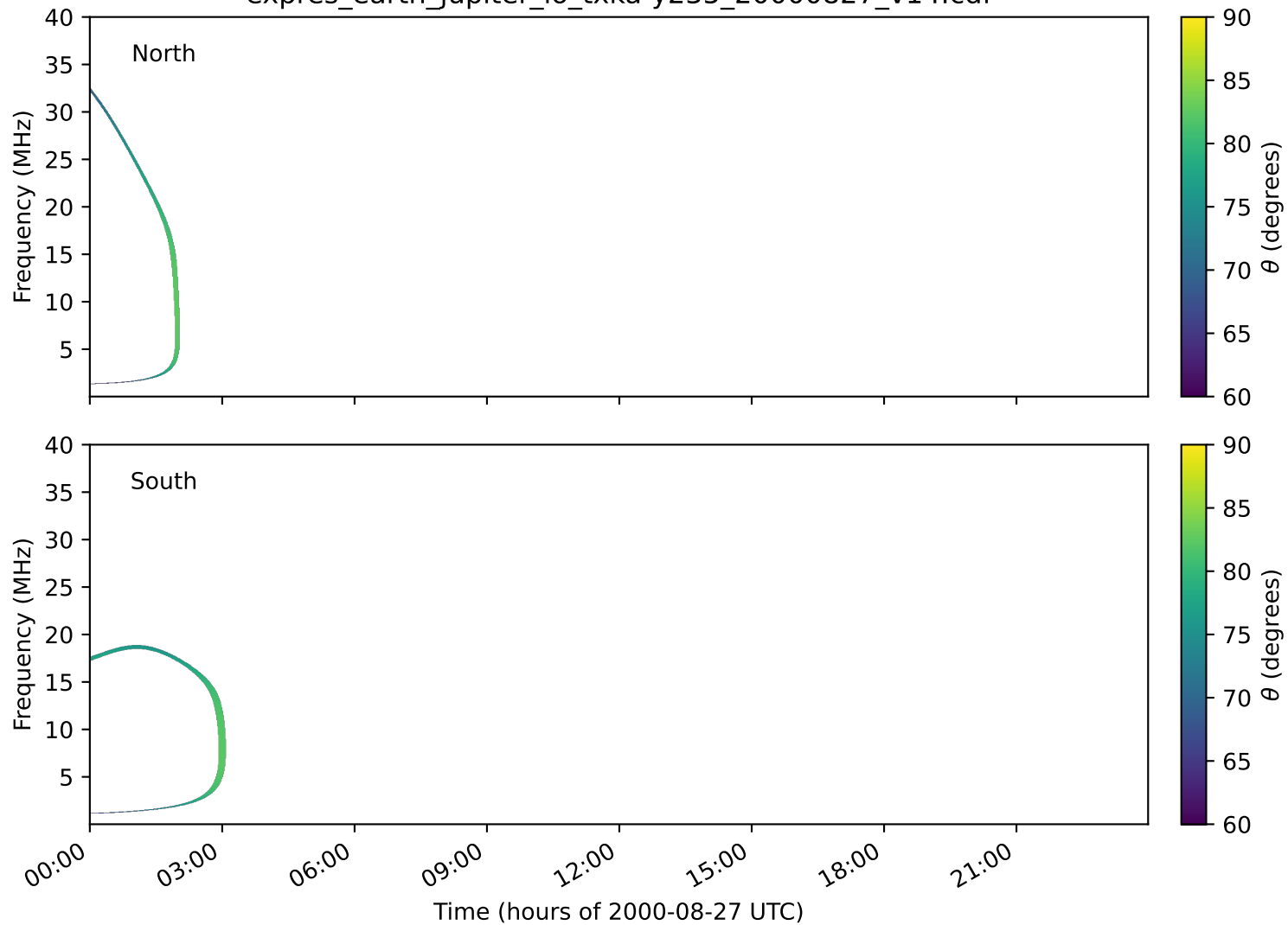
expres_earth_jupiter_io_txka-y235_20000827_v14.cdf
