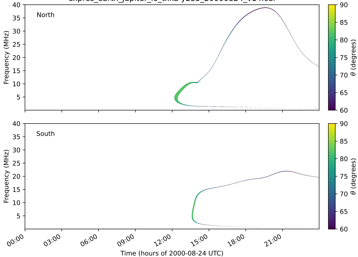
expres_earth_jupiter_io_txka-y235_20000824_v14.cdf
