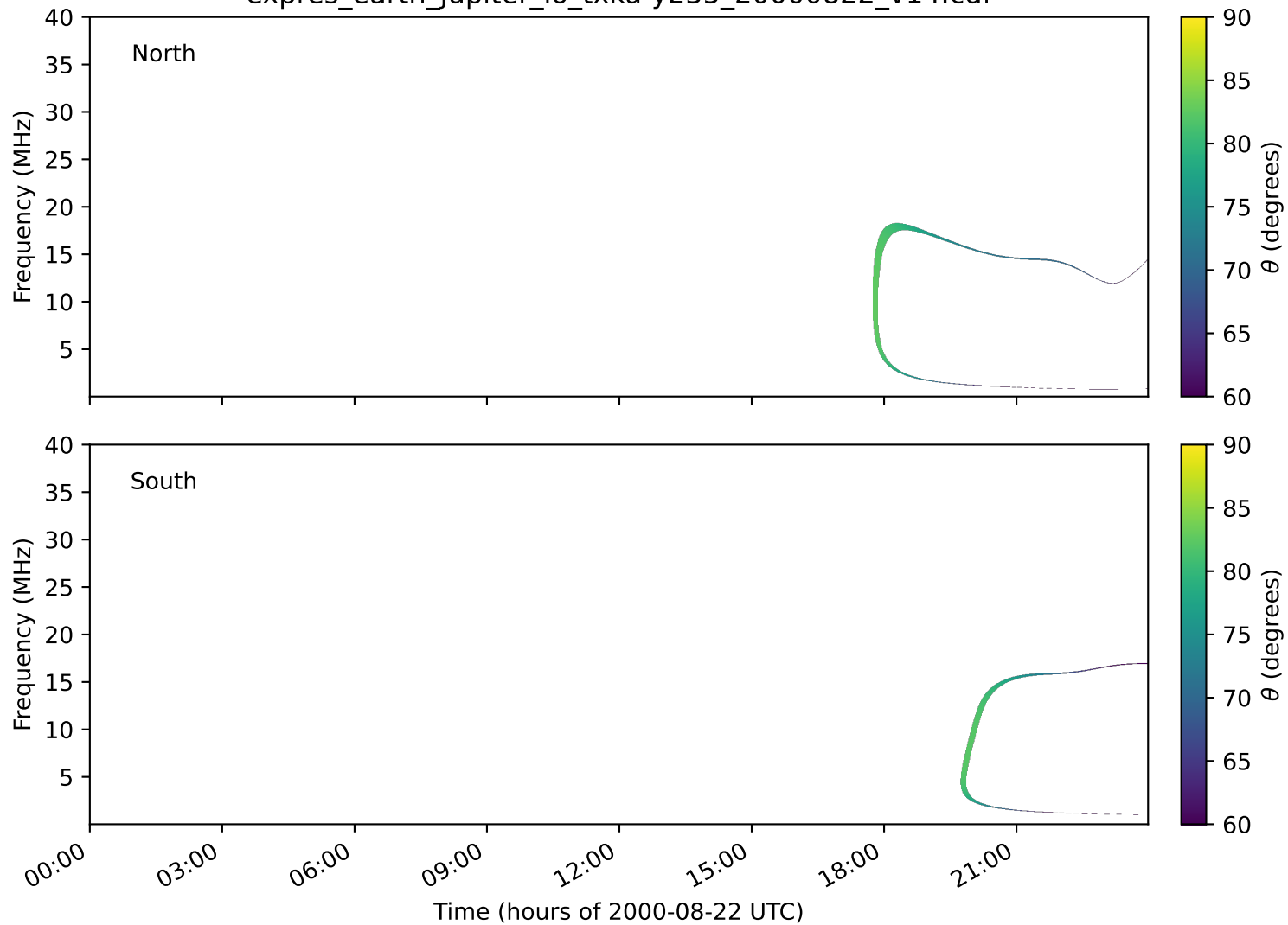
expres_earth_jupiter_io_txka-y235_20000822_v14.cdf
