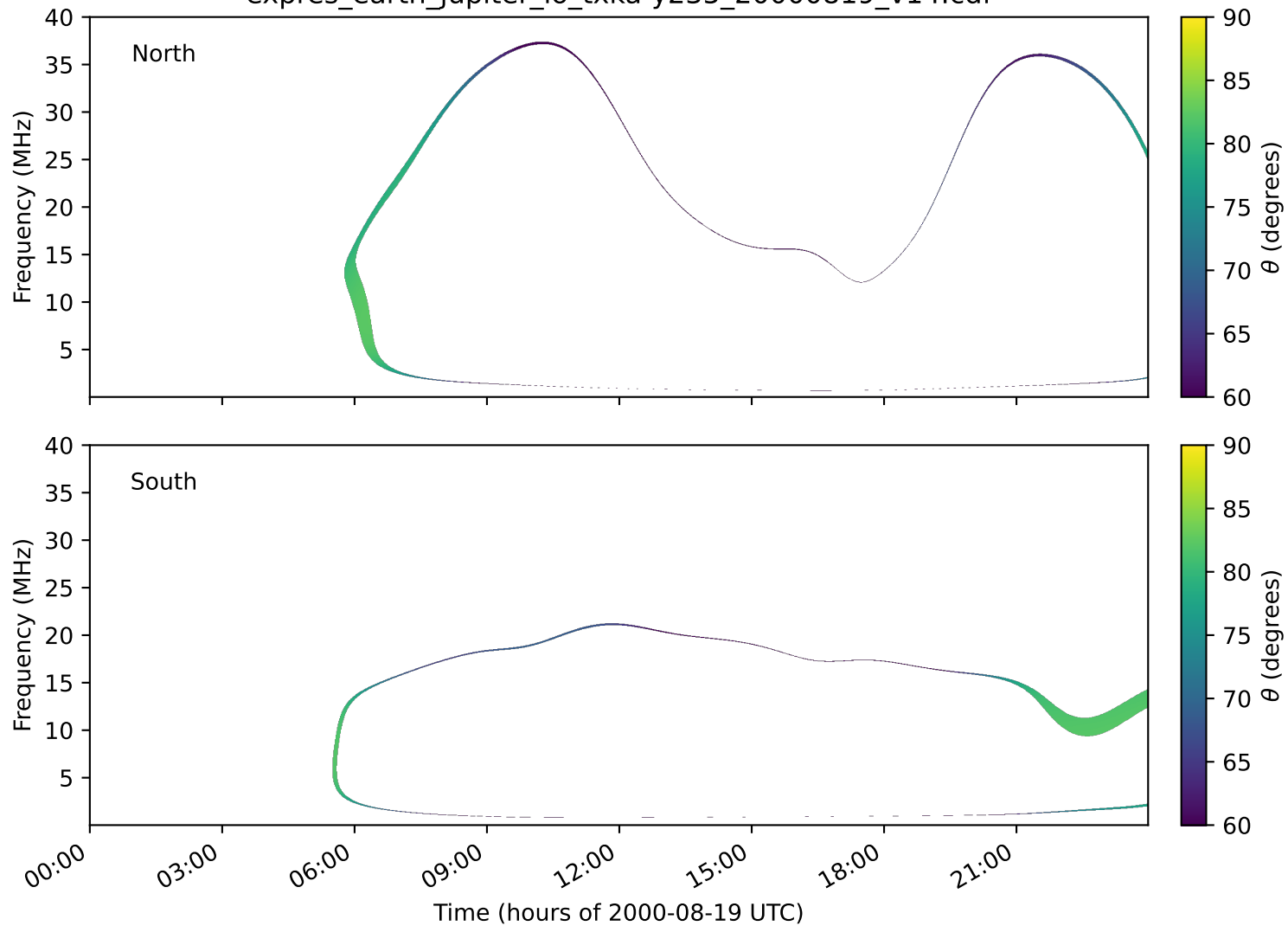
expres_earth_jupiter_io_txka-y235_20000819_v14.cdf
