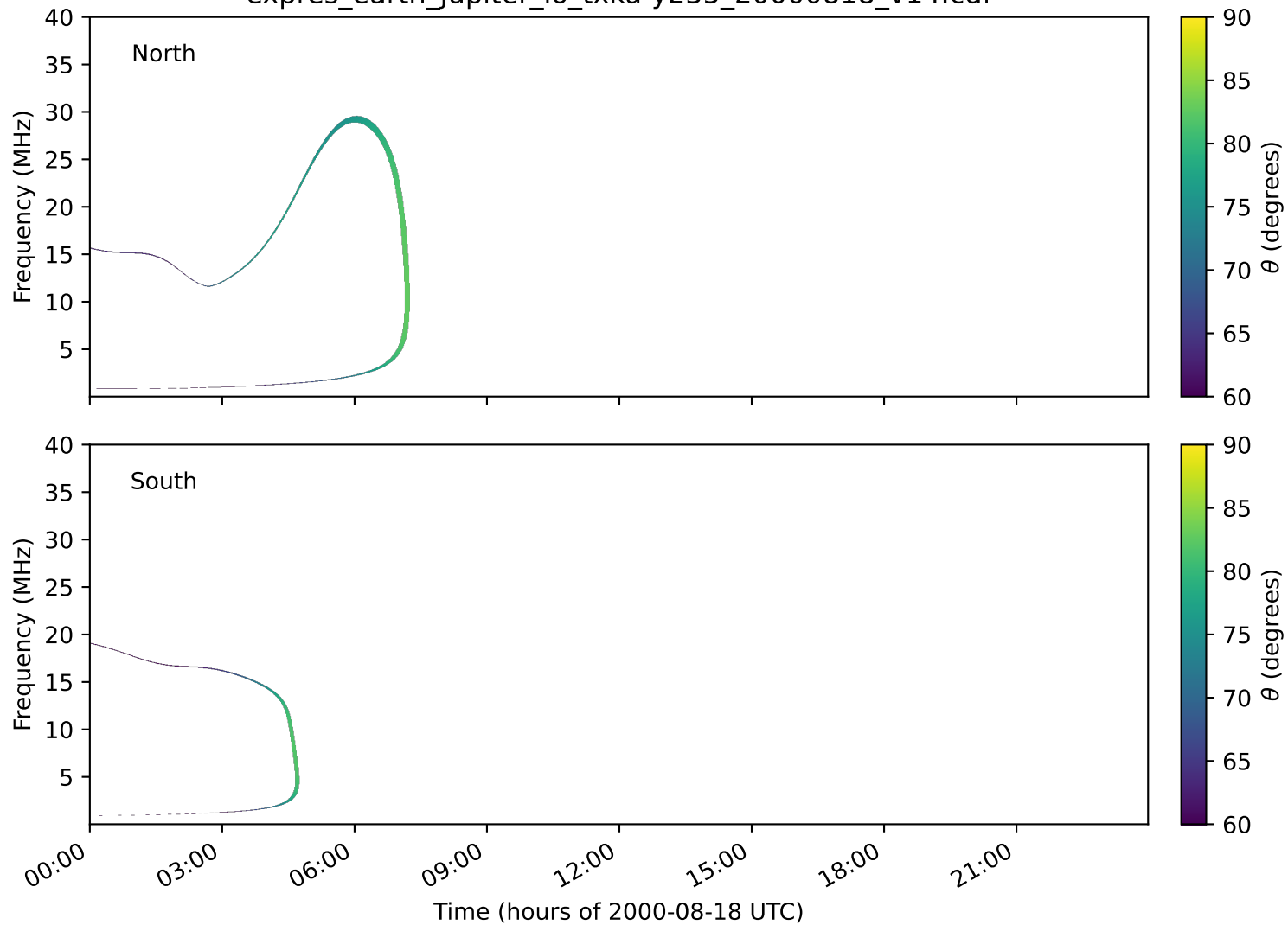
expres_earth_jupiter_io_txka-y235_20000818_v14.cdf
