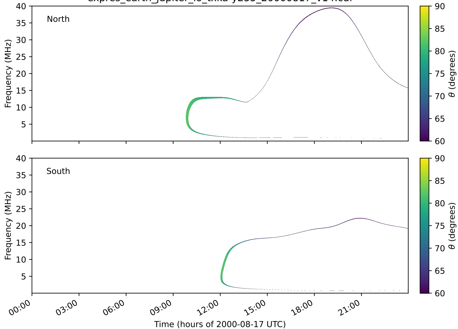
expres_earth_jupiter_io_txka-y235_20000817_v14.cdf
