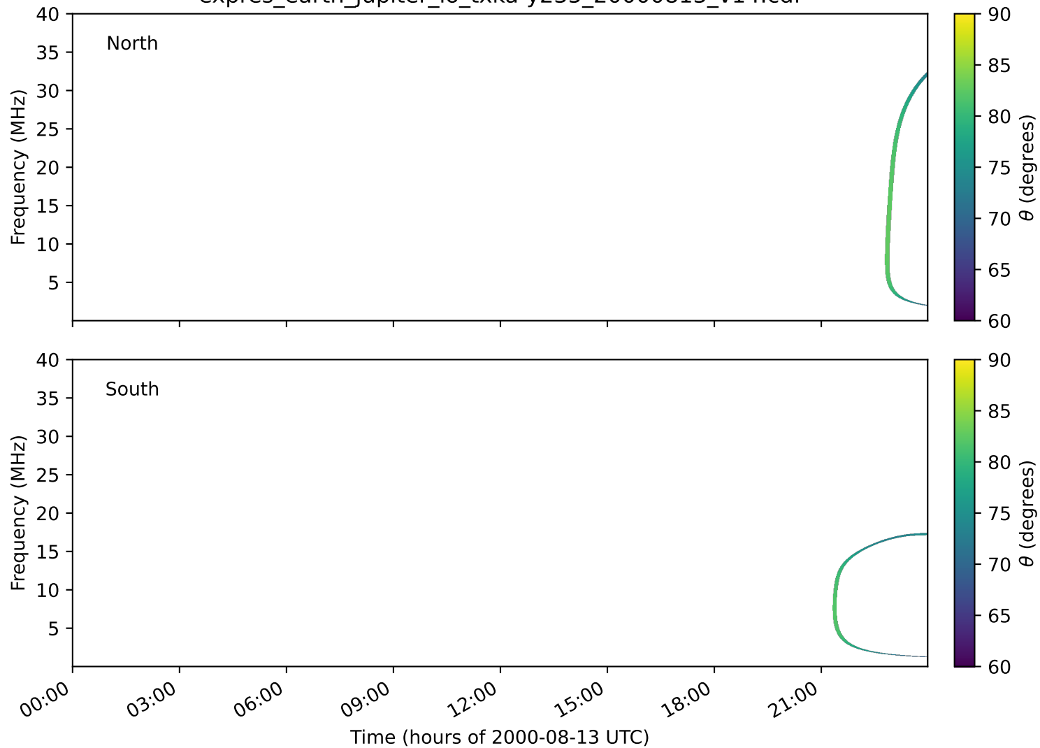
expres_earth_jupiter_io_txka-y235_20000813_v14.cdf
