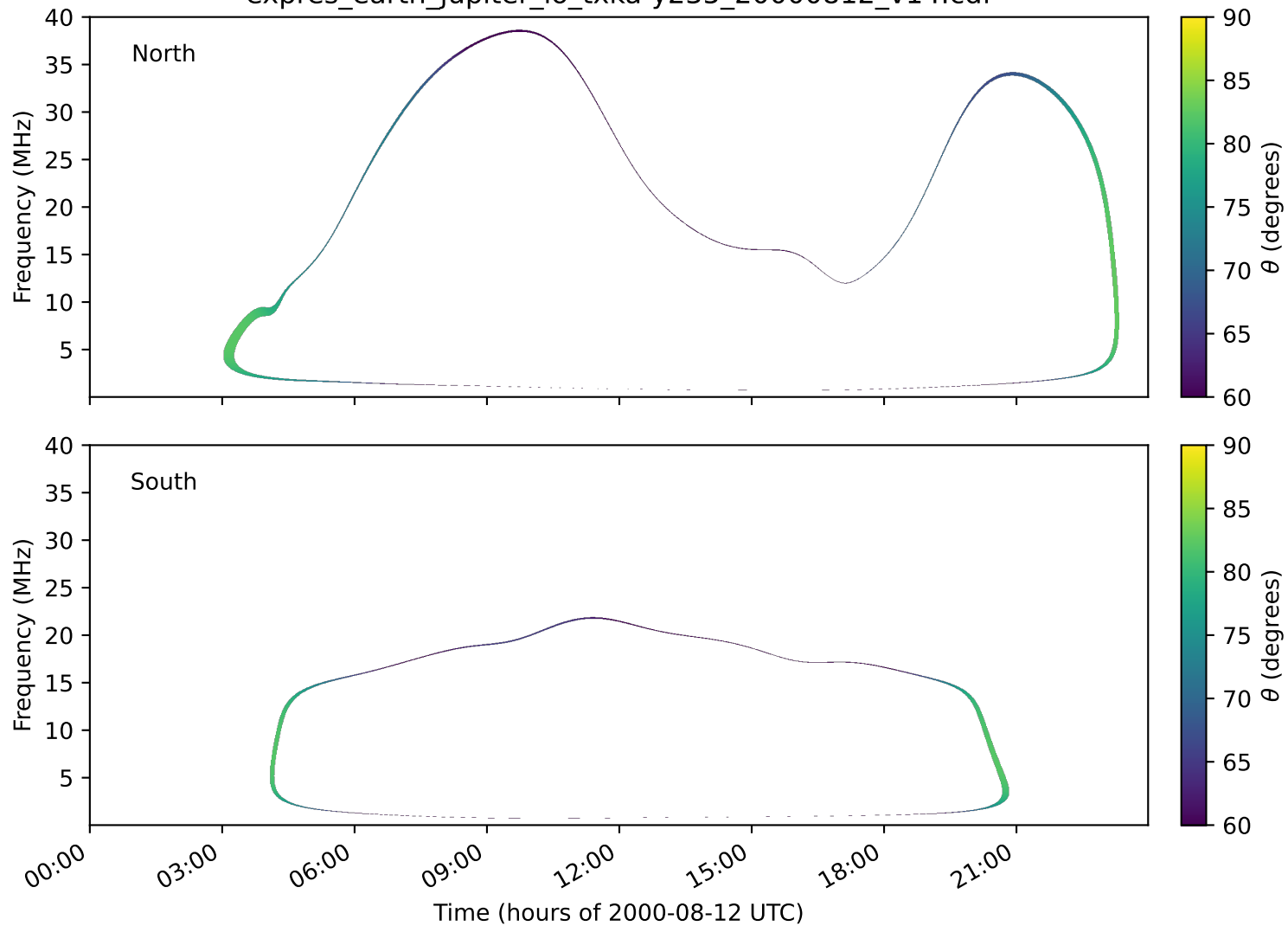
expres_earth_jupiter_io_txka-y235_20000812_v14.cdf
