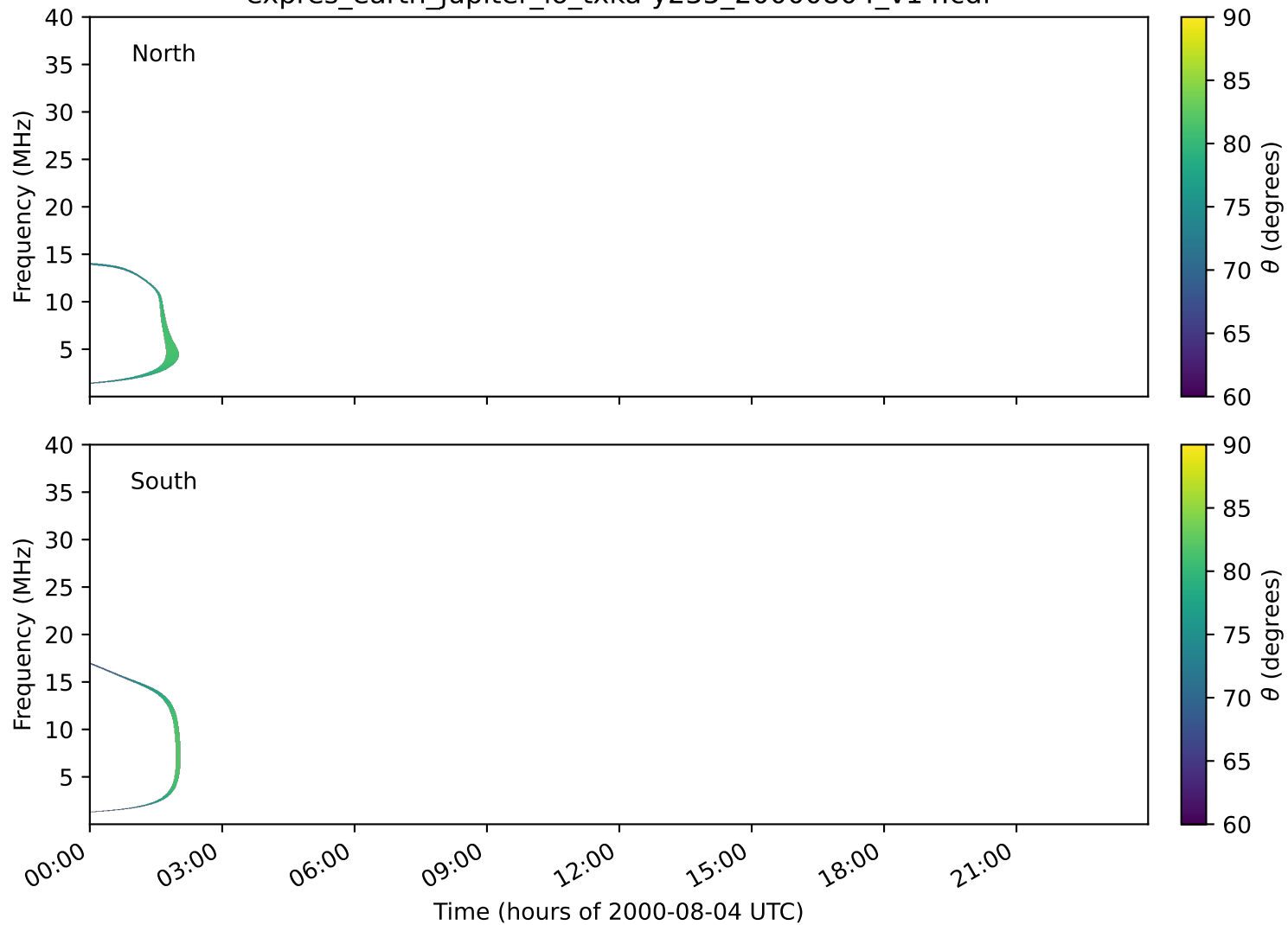
expres_earth_jupiter_io_txka-y235_20000804_v14.cdf
