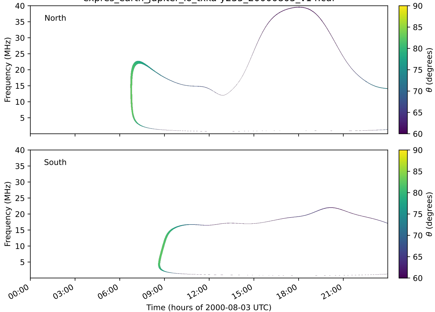
expres_earth_jupiter_io_txka-y235_20000803_v14.cdf
