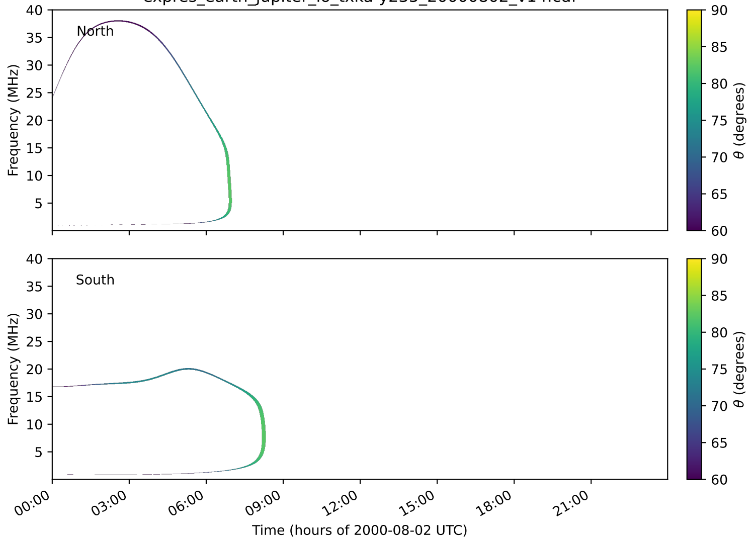
expres_earth_jupiter_io_txka-y235_20000802_v14.cdf
