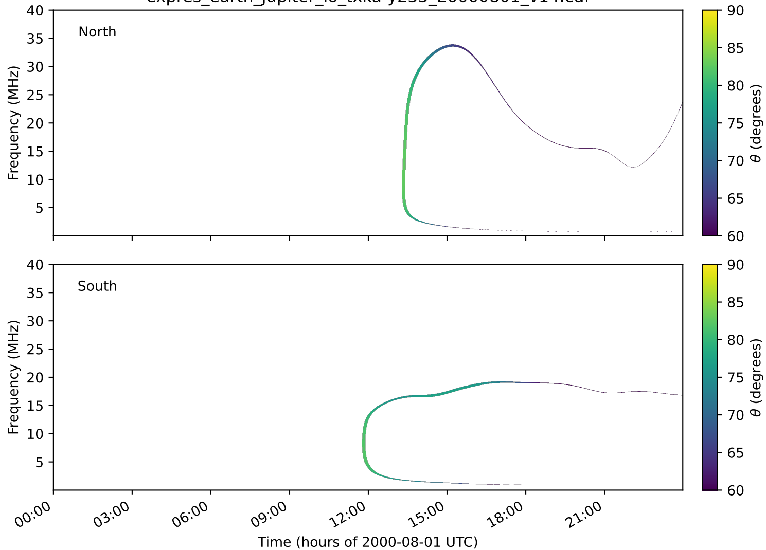
expres_earth_jupiter_io_txka-y235_20000801_v14.cdf
