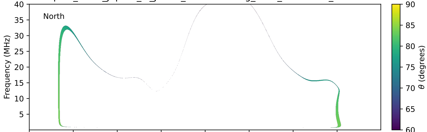
expres_earth_jupiter_io_jrm33_lossc-wid1deg_3kev_20000828_v11.cdf
