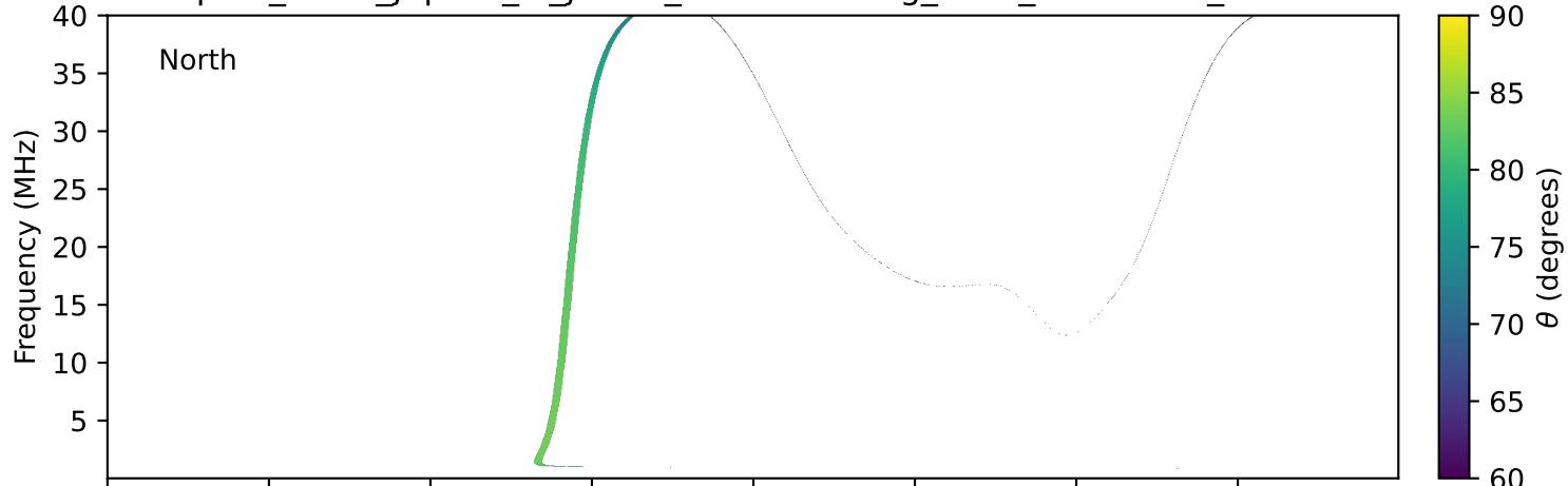
expres_earth_jupiter_io_jrm33_lossc-wid1deg_3kev_20000826_v11.cdf
