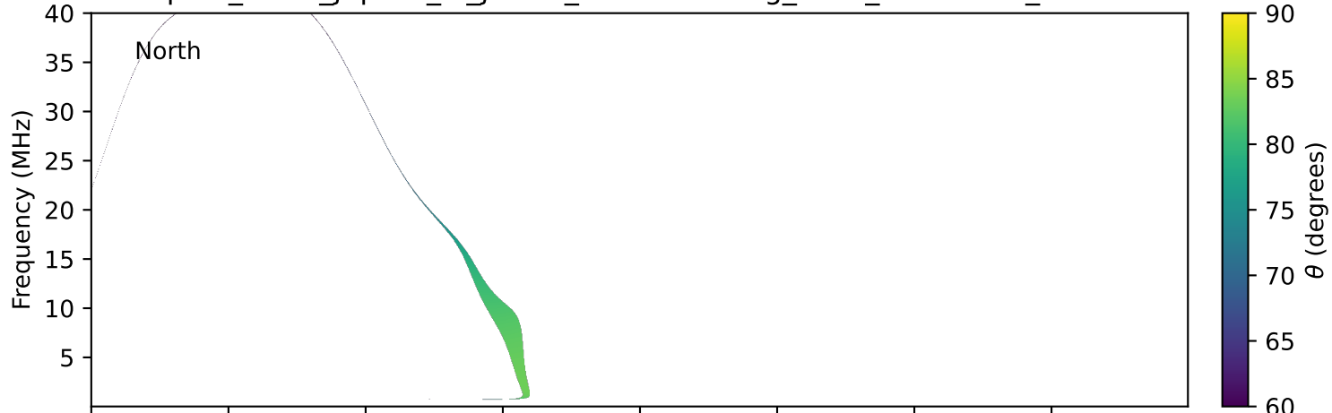
expres_earth_jupiter_io_jrm33_lossc-wid1deg_3kev_20000809_v11.cdf
