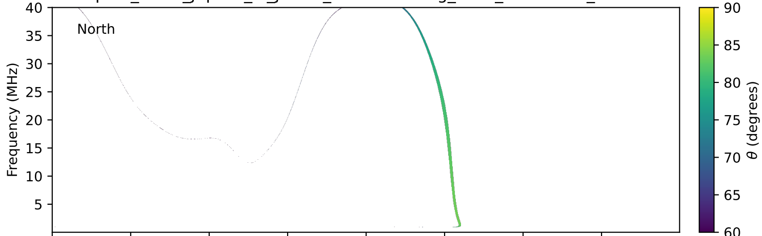
expres_earth_jupiter_io_jrm33_lossc-wid1deg_3kev_20000807_v11.cdf
