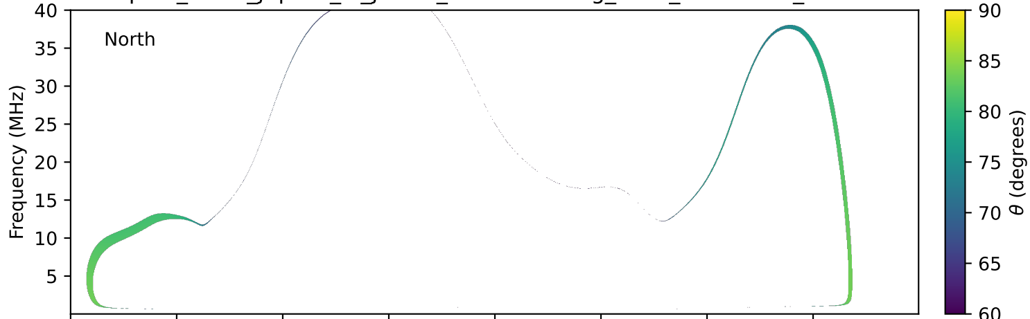
expres_earth_jupiter_io_jrm33_lossc-wid1deg_3kev_20000805_v11.cdf
