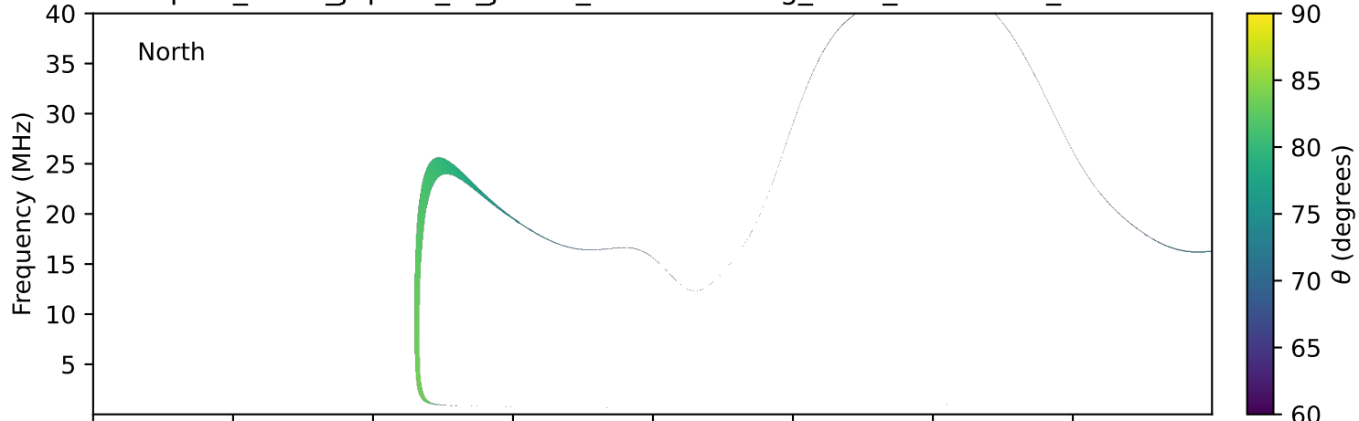
expres_earth_jupiter_io_jrm33_lossc-wid1deg_3kev_20000803_v11.cdf
