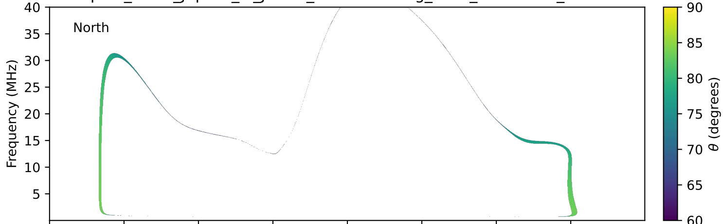
expres_earth_jupiter_io_jrm09_lossc-wid1deg_3kev_20000828_v11.cdf
