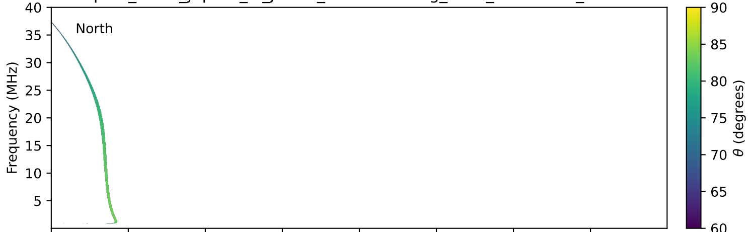
expres_earth_jupiter_io_jrm09_lossc-wid1deg_3kev_20000827_v11.cdf
