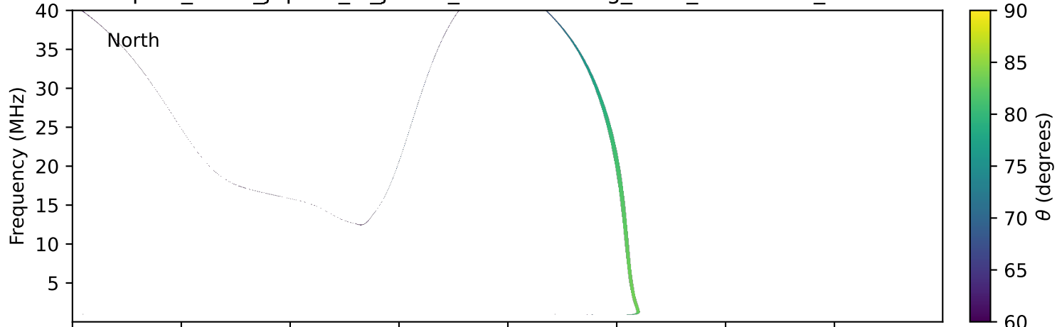
expres_earth_jupiter_io_jrm09_lossc-wid1deg_3kev_20000807_v11.cdf
