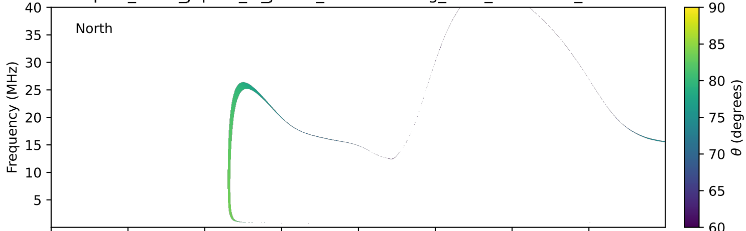
expres_earth_jupiter_io_jrm09_lossc-wid1deg_3kev_20000803_v11.cdf
