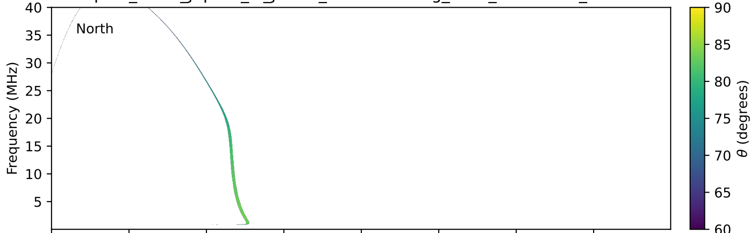
expres_earth_jupiter_io_jrm09_lossc-wid1deg_3kev_20000802_v11.cdf
