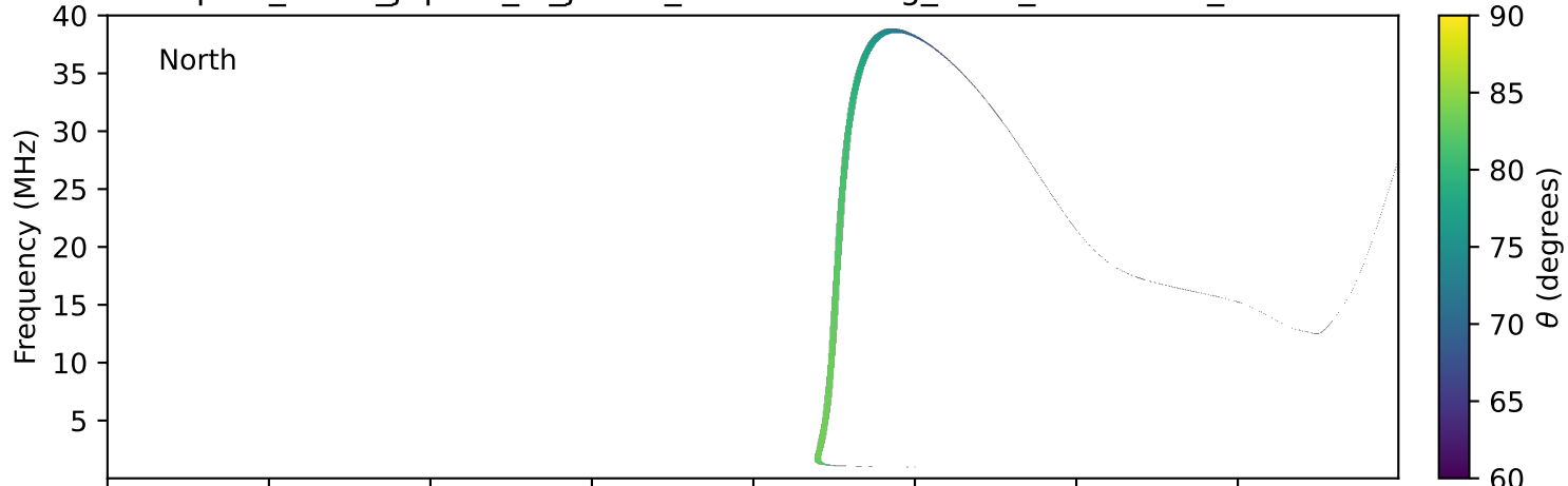
expres_earth_jupiter_io_jrm09_lossc-wid1deg_3kev_20000801_v11.cdf
