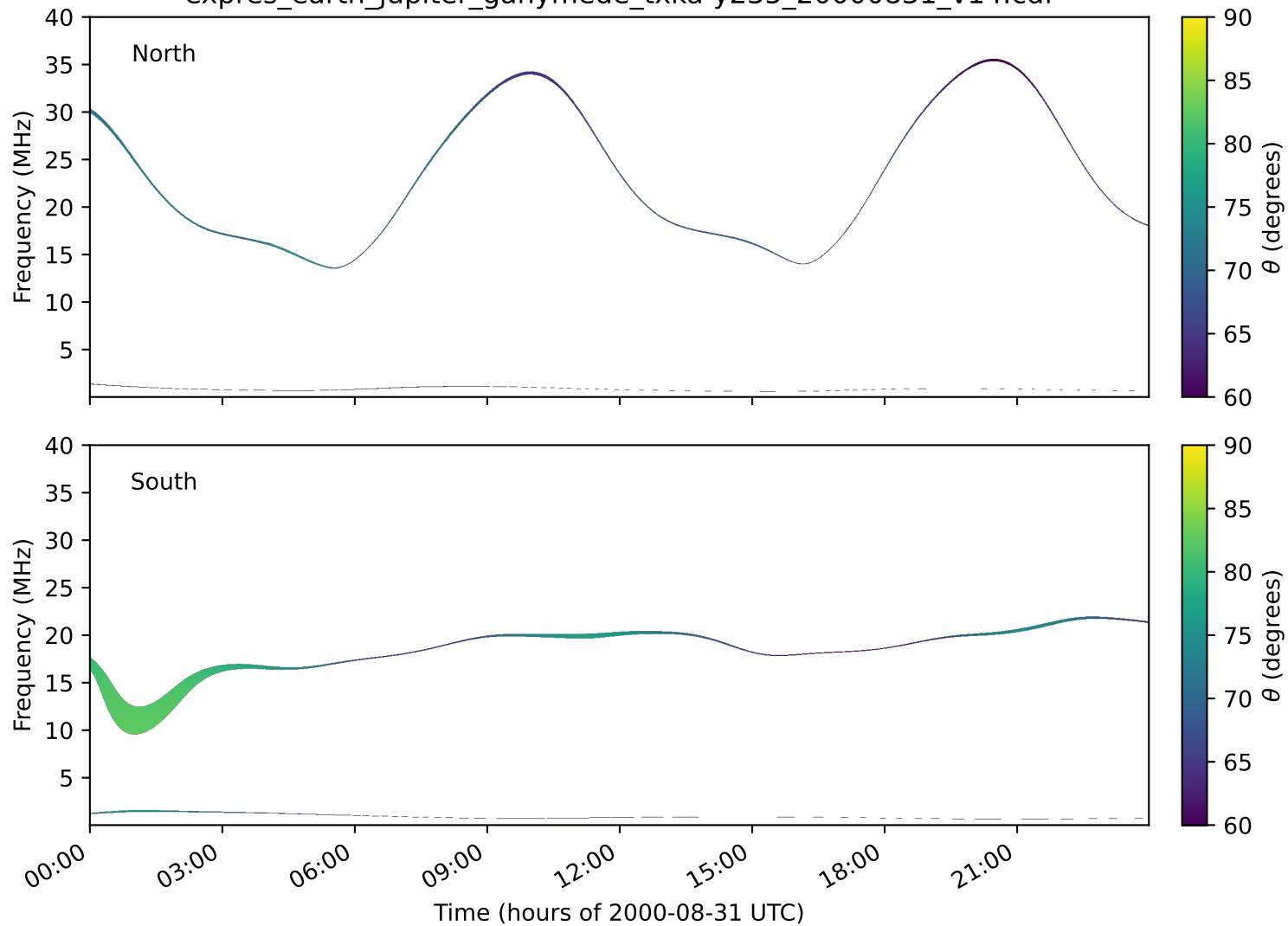
expres_earth_jupiter_ganymede_txka-y235_20000831_v14.cdf
