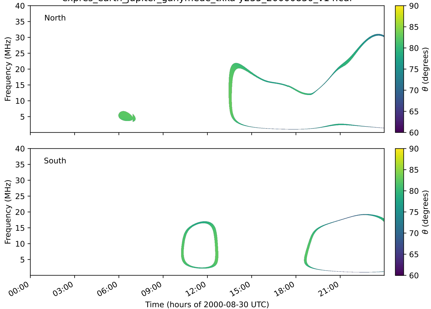
expres_earth_jupiter_ganymede_txka-y235_20000830_v14.cdf
