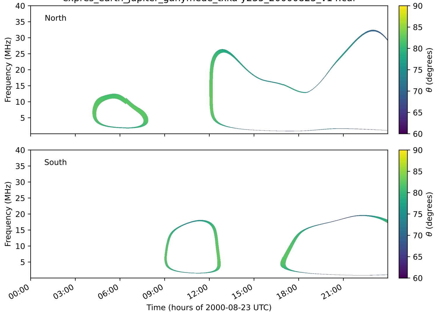
expres_earth_jupiter_ganymede_txka-y235_20000823_v14.cdf
