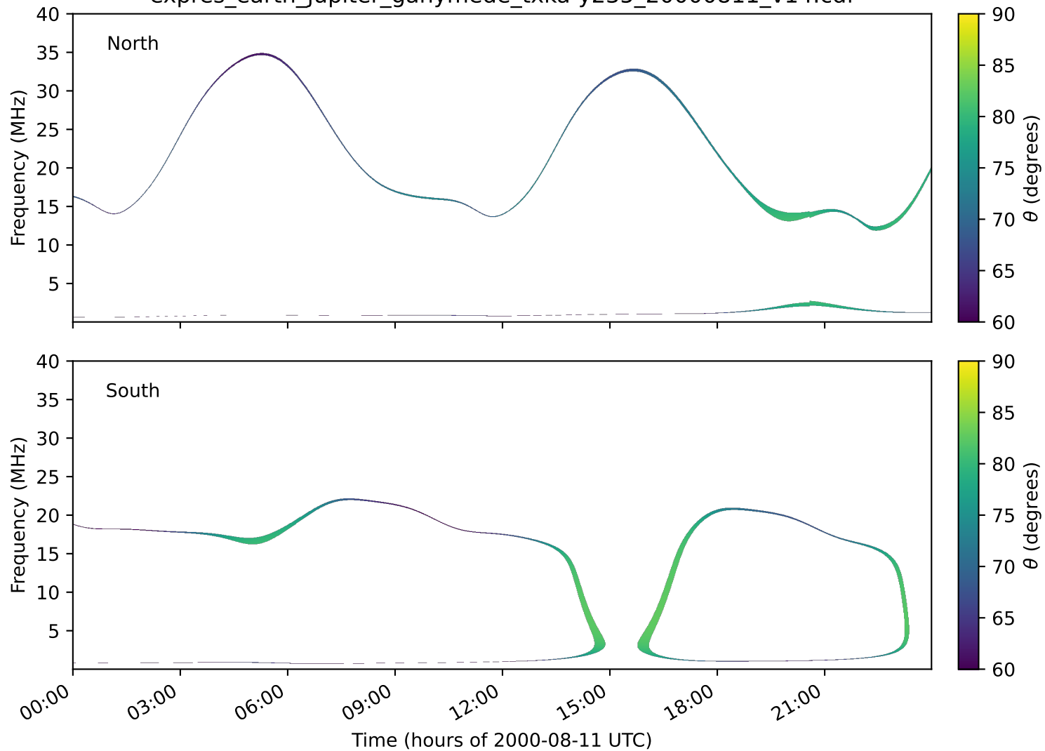
expres_earth_jupiter_ganymede_txka-y235_20000811_v14.cdf
