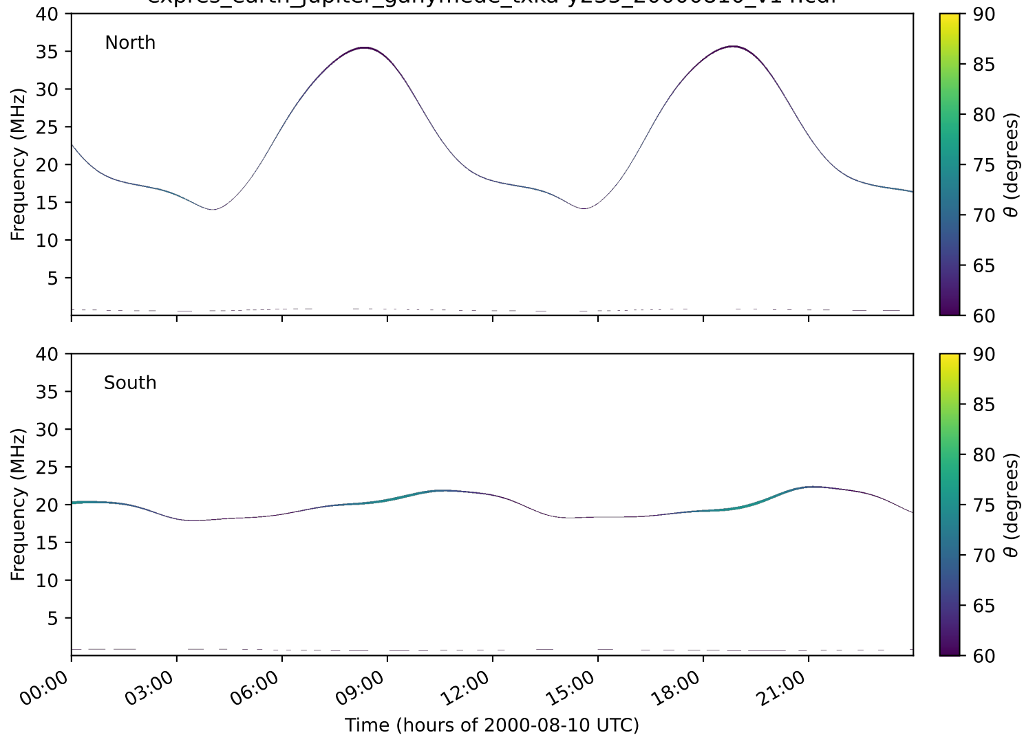
expres_earth_jupiter_ganymede_txka-y235_20000810_v14.cdf
