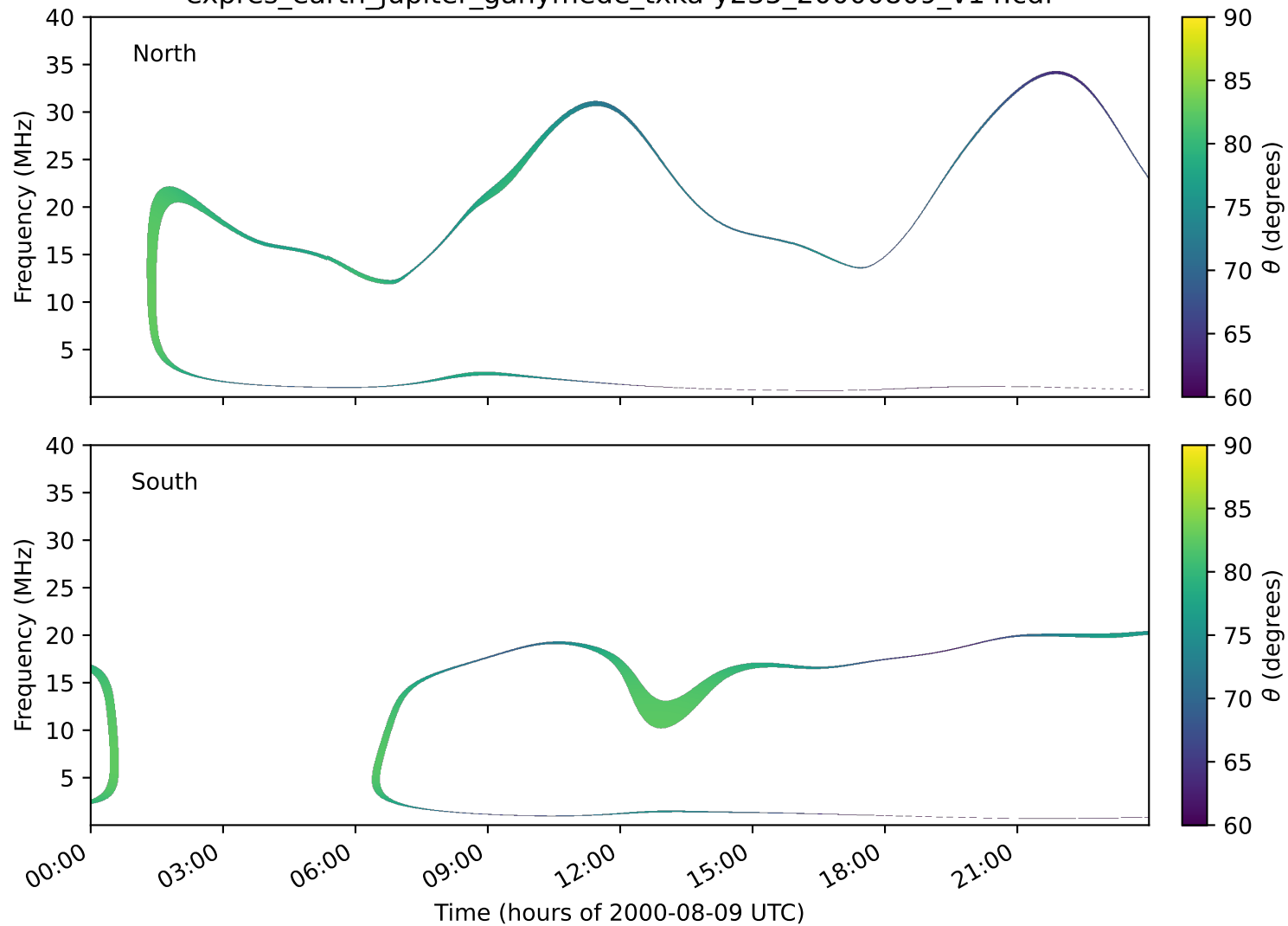
expres_earth_jupiter_ganymede_txka-y235_20000809_v14.cdf
