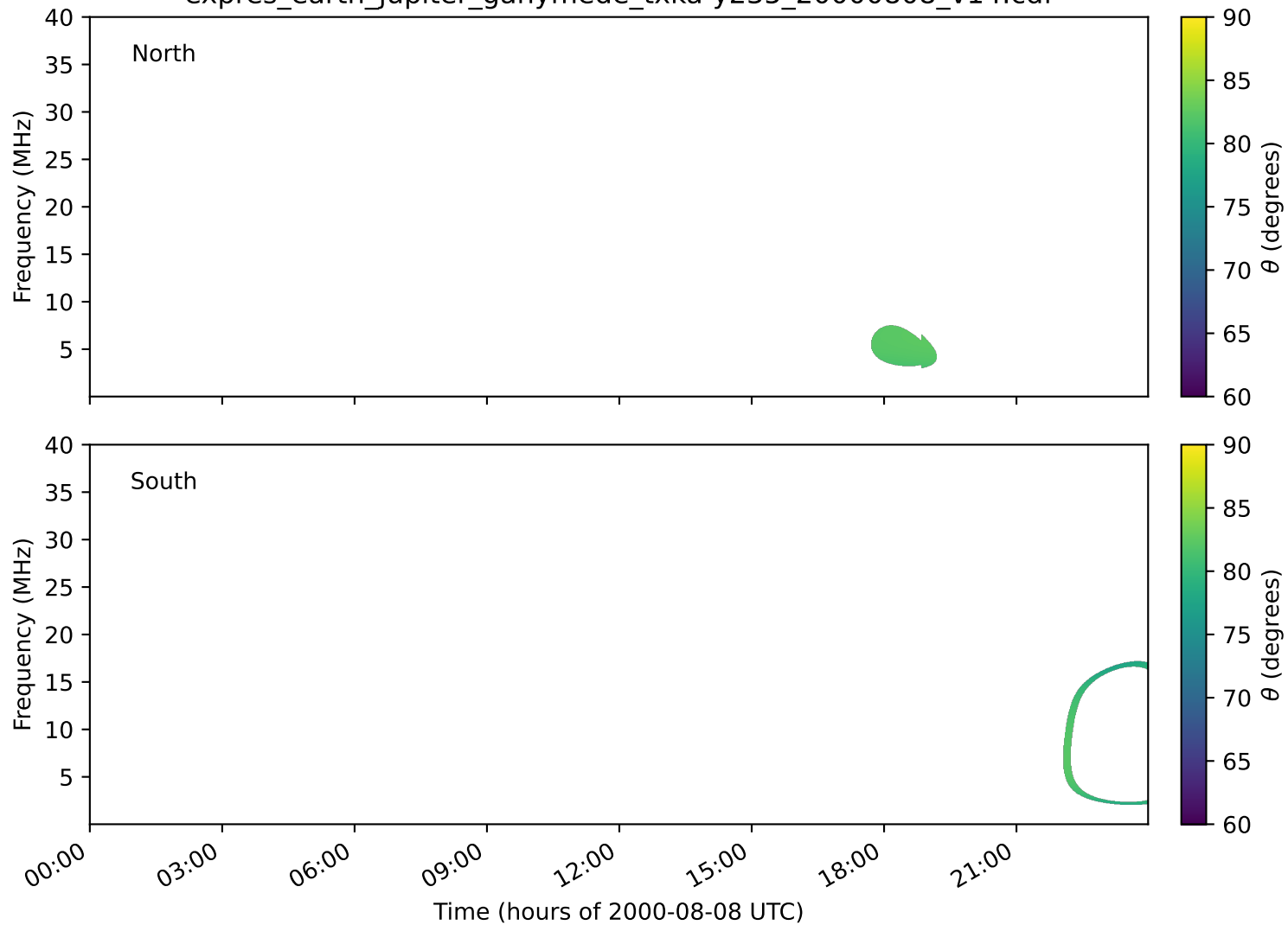
expres_earth_jupiter_ganymede_txka-y235_20000808_v14.cdf
