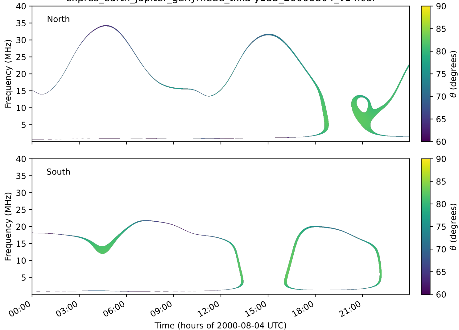
expres_earth_jupiter_ganymede_txka-y235_20000804_v14.cdf
