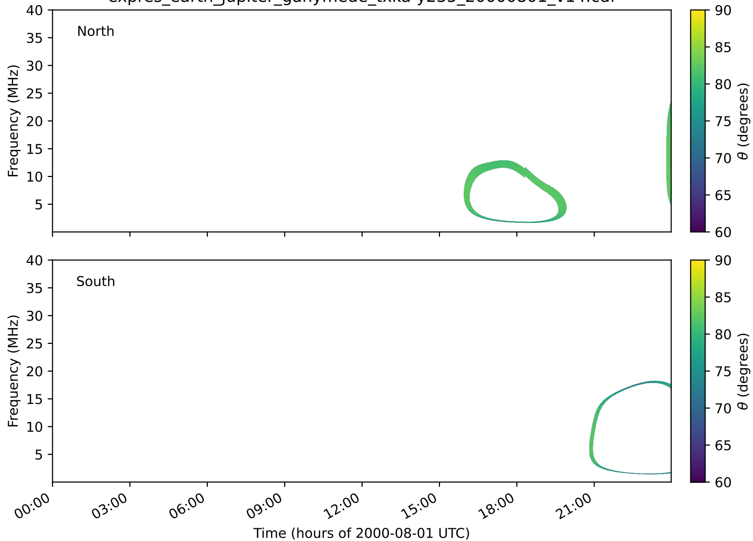
expres_earth_jupiter_ganymede_txka-y235_20000801_v14.cdf
