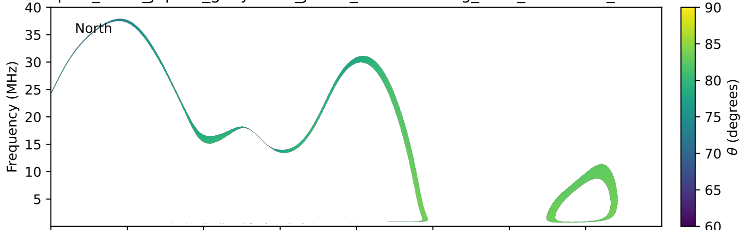
expres_earth_jupiter_ganymede_jrm33_lossc-wid1deg_3kev_20000819_v11.cdf
