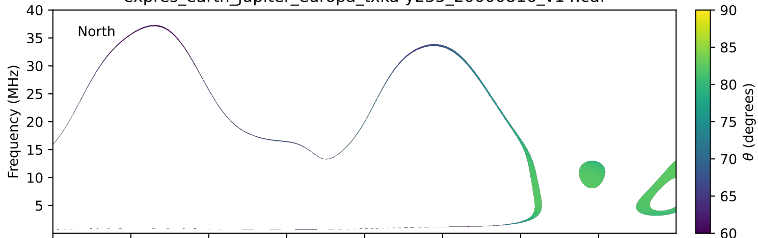
expres_earth_jupiter_europa_txka-y235_20000816_v14.cdf
