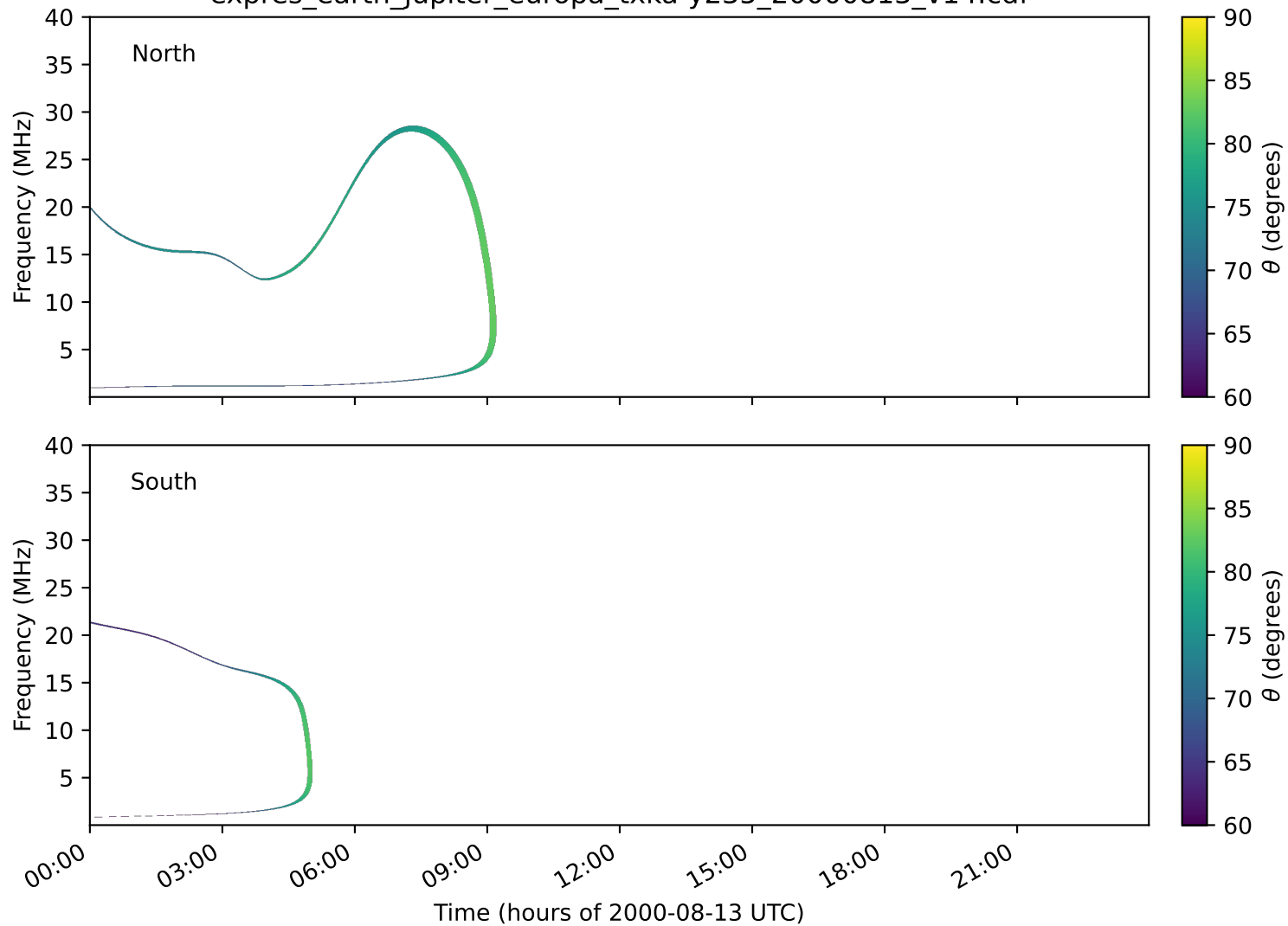
expres_earth_jupiter_europa_txka-y235_20000813_v14.cdf
