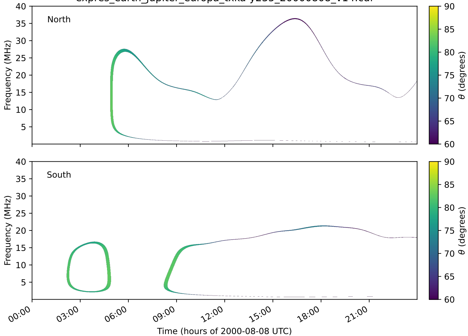
expres_earth_jupiter_europa_txka-y235_20000808_v14.cdf
