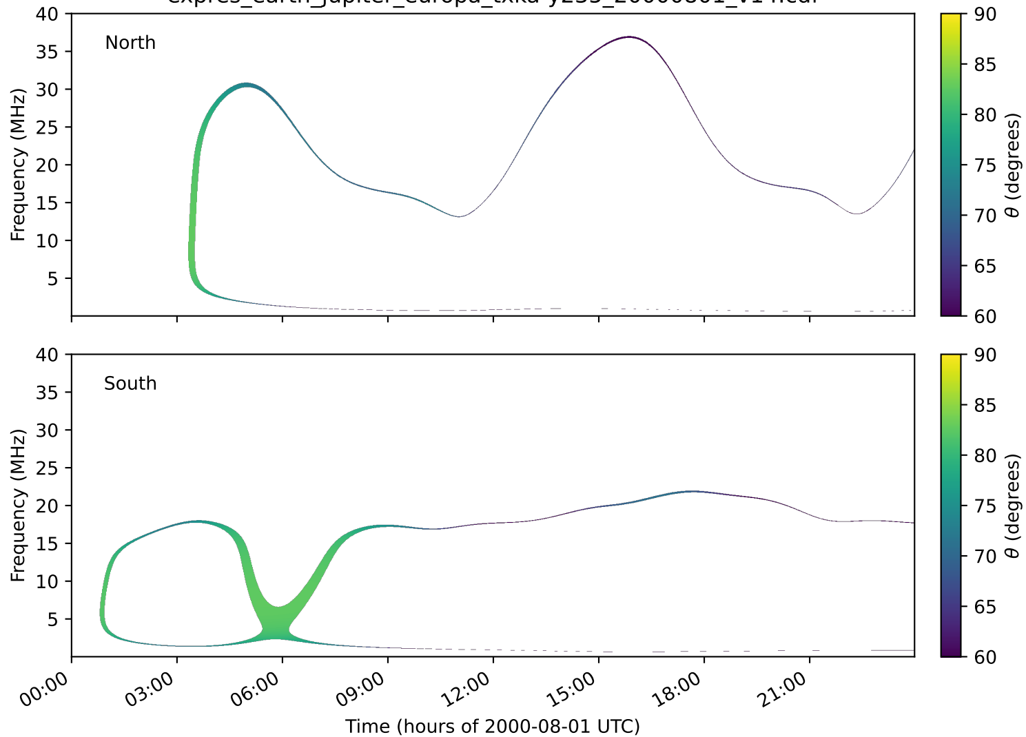
expres_earth_jupiter_europa_txka-y235_20000801_v14.cdf
