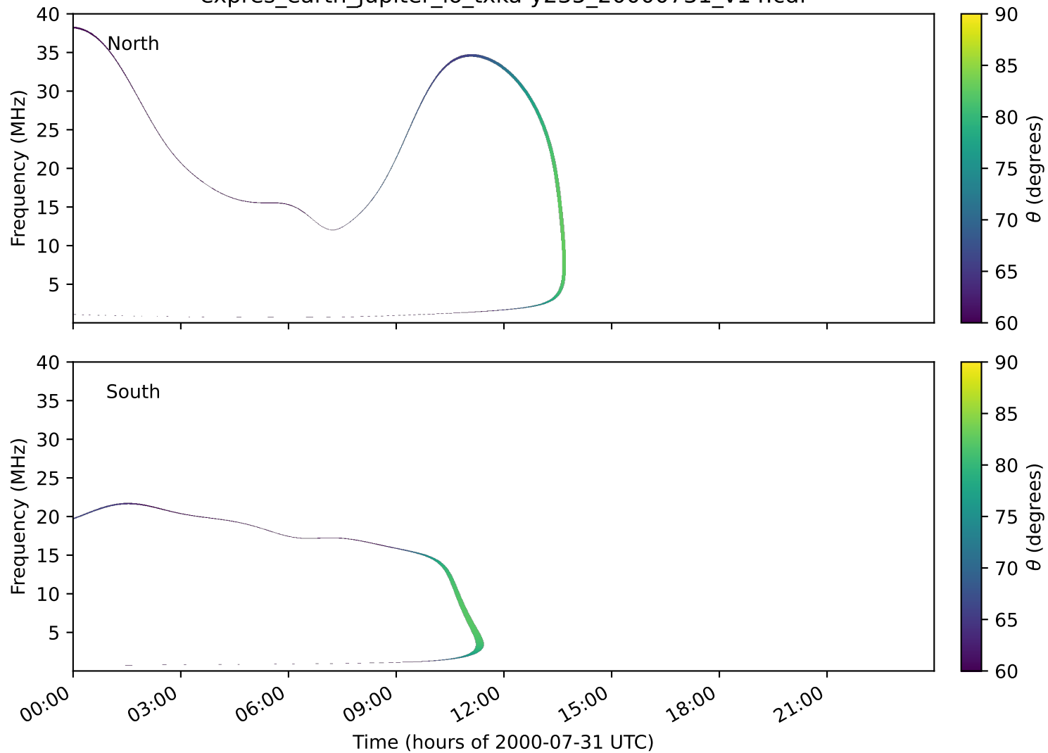
expres_earth_jupiter_io_txka-y235_20000731_v14.cdf
