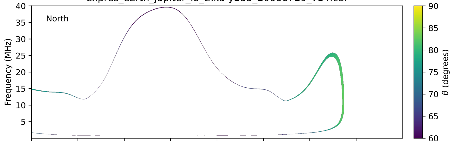
expres_earth_jupiter_io_txka-y235_20000729_v14.cdf
