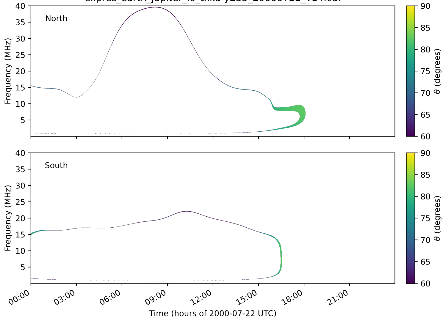
expres_earth_jupiter_io_txka-y235_20000722_v14.cdf
